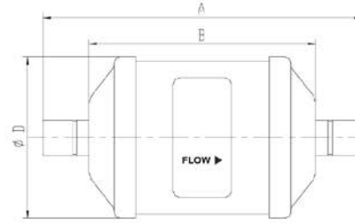
Solder Connection
