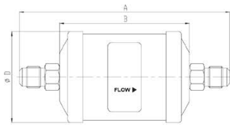
Flare Connection
