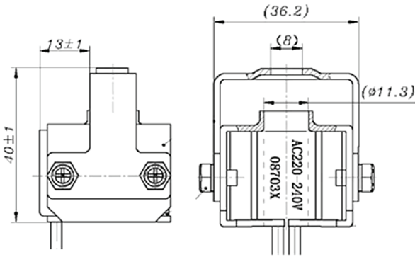
Drawing 2: FQA-55007
